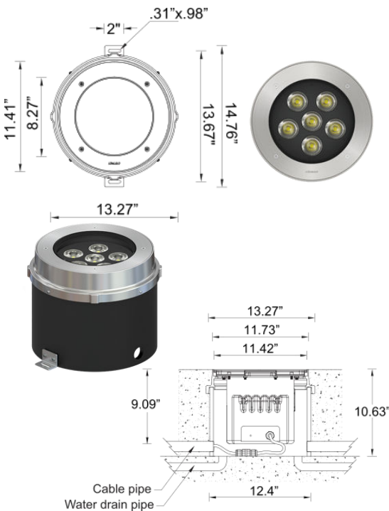
Mounting Detail
